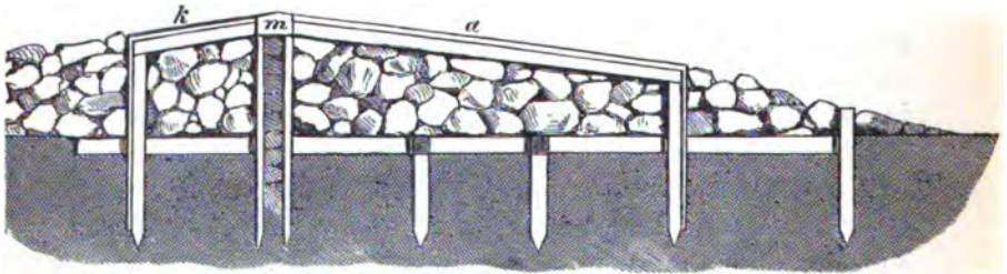
Fig. 244.—Overflow weir with slight fall.
